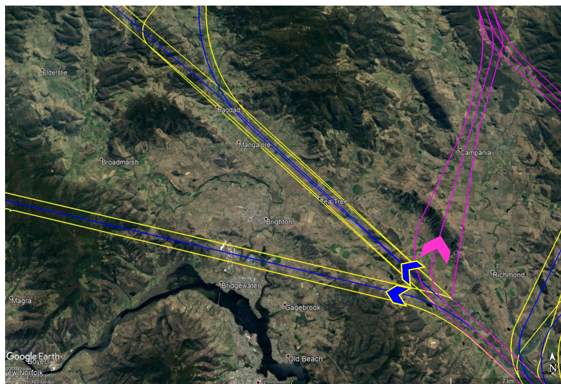
Figure 2: Runway 30 Operations
