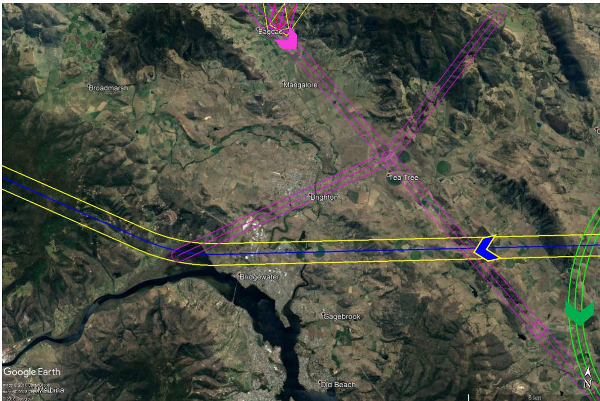
Figure 1: Runway 12 Operations
